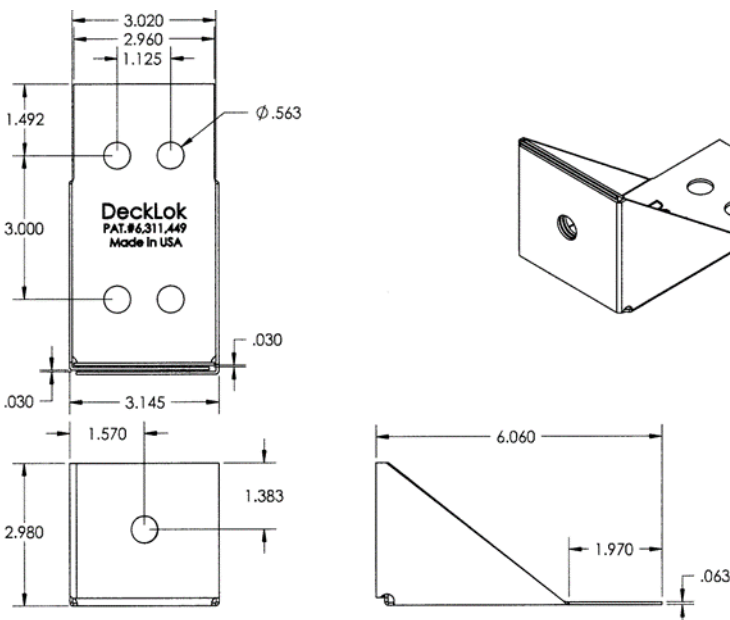
FIGURE 1—DeckLok connector Geometry and Dimensions
